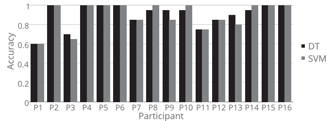
Fig. 14. Classification accuracy by participant (tilt-based solution).
